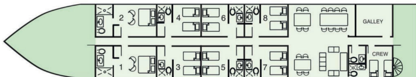
MAIN DECK
